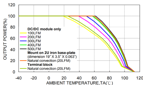
Temperatur-Derating / Temperature de-rating PMDP200 48S05UHB
